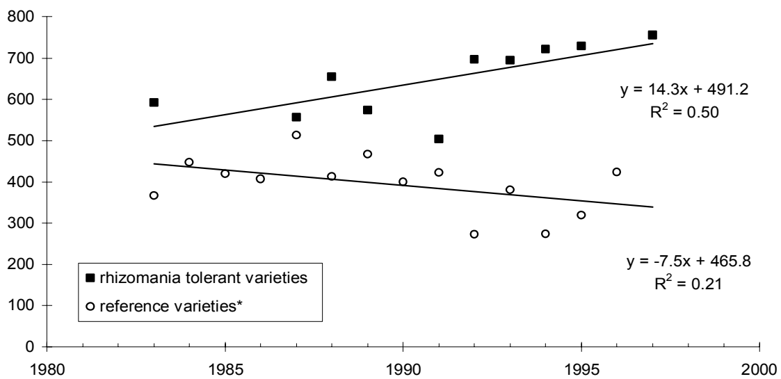
Figure 2: Development of the variety performance of sugar beets in rhizomania infested areas: sugar beet yield [dt/ha]; with x_{1980} = 0
