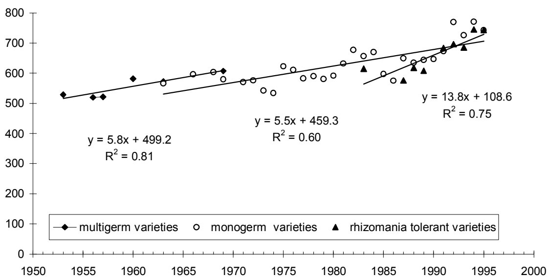
Figure 1: Development of the genetic potential of sugar beets by variety attribute sugar beet yield [dt/ha]
