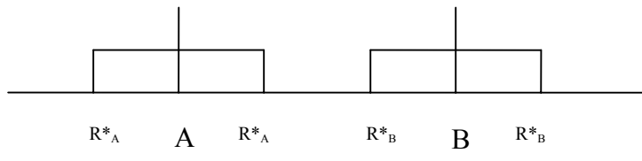
Figure 1: Local monopoly
