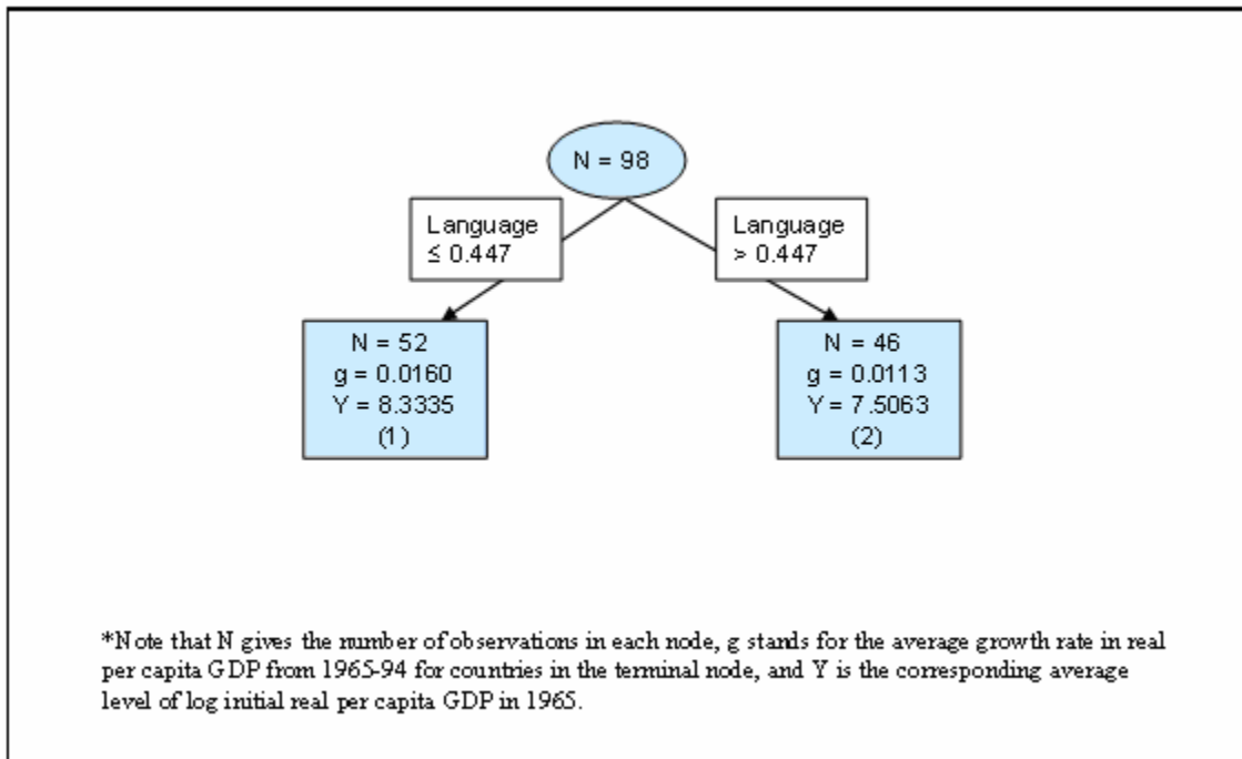
Figure 3(a)*: Tree diagram for TR baseline model
