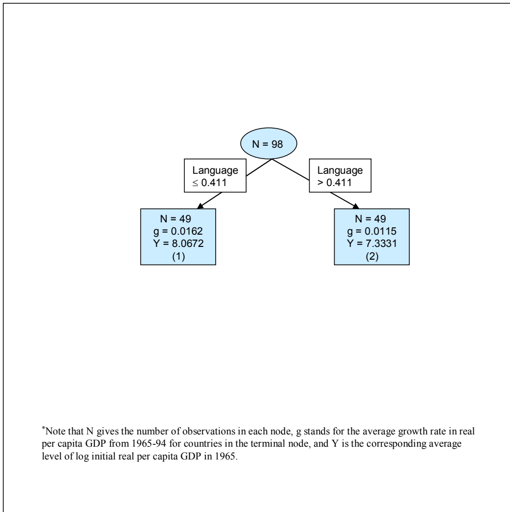
Figure 2(a)*: Tree diagram for BTREED baseline model
