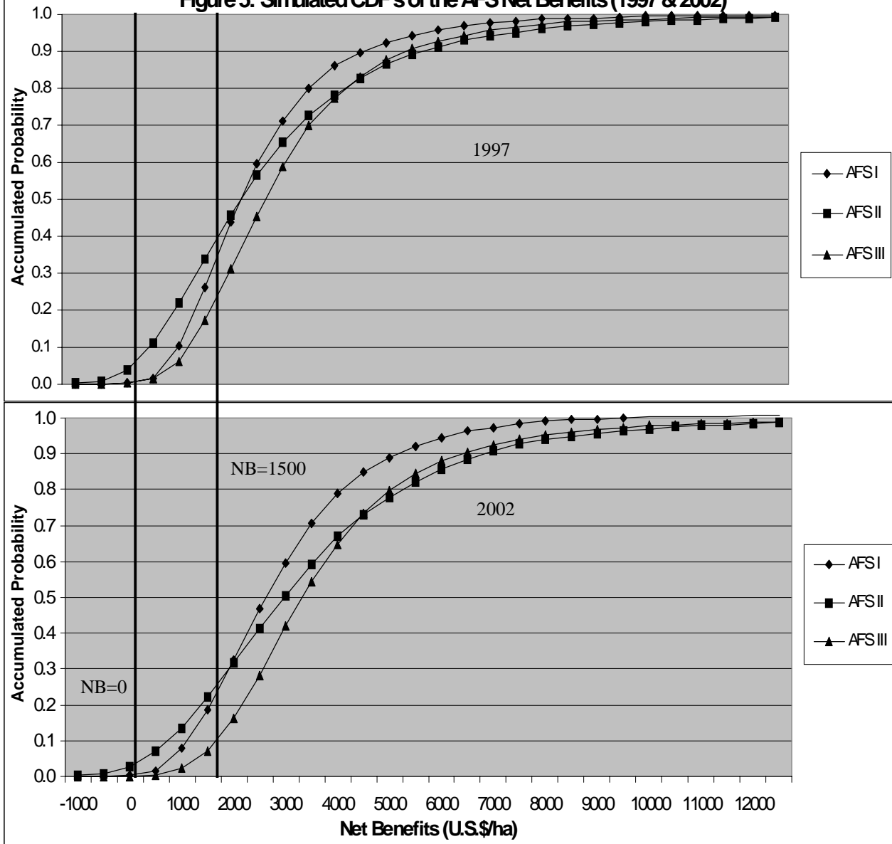
Figure 5: Simulated CDF's of the AFS Net Benefits (1997 & 2002)
