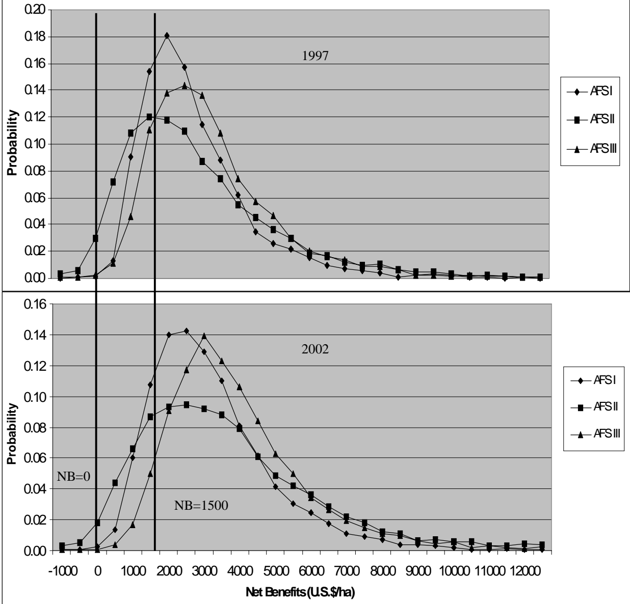
Figure 4: Simulated pdf's for the AFS Net Benefits (1997 & 2002)
